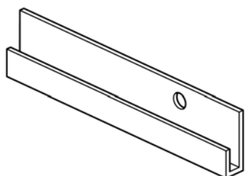
STAS j-rail 7x20mm - 25 kg/m 1
