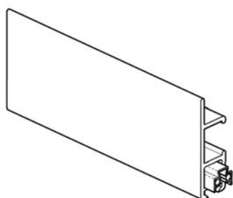
STAS multirail max 12V 11x38 mm - 45 kg/m 1
